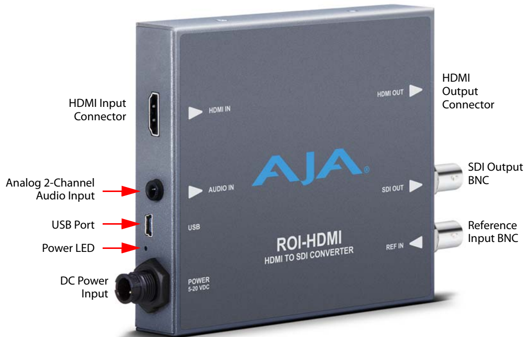
Figure 2. ROI-HDMI Converter/Scaler
